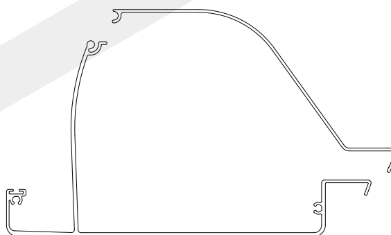
Tampa e lâmina do motor Capot moteur et lame Engine cover and louver
