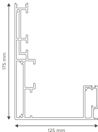
Estrutura/Caleira Structure/Gouttière Structure/Gutter
